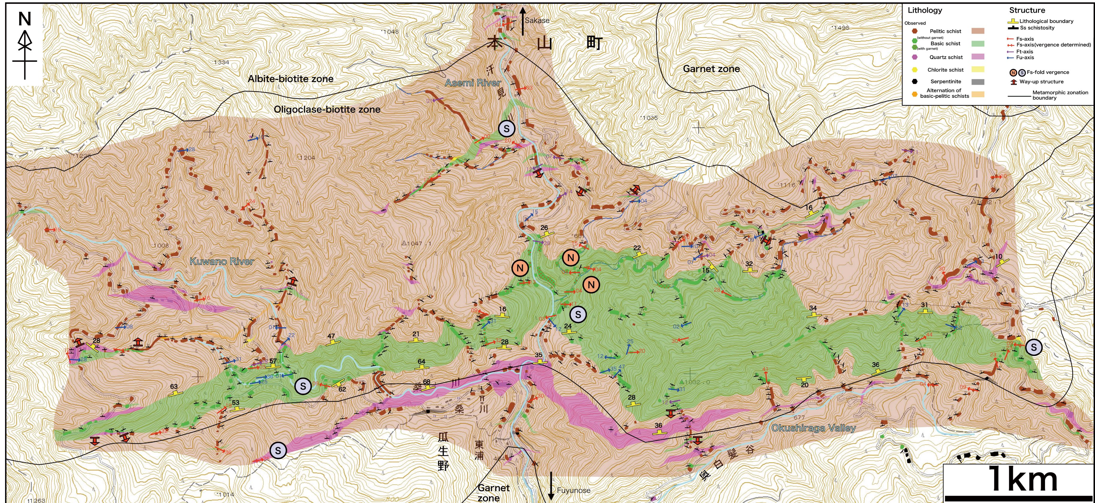
Lithological map of the study area with distribution of rocks and structures observed by field study, and orientation of the lithological boundary measured by geological mapping, which is drawn over a topographical map in Japanese language. The outer frame is the same size and location as Figure 3. Metamorphic zonation boundaries are taken from Higashino (1990).
