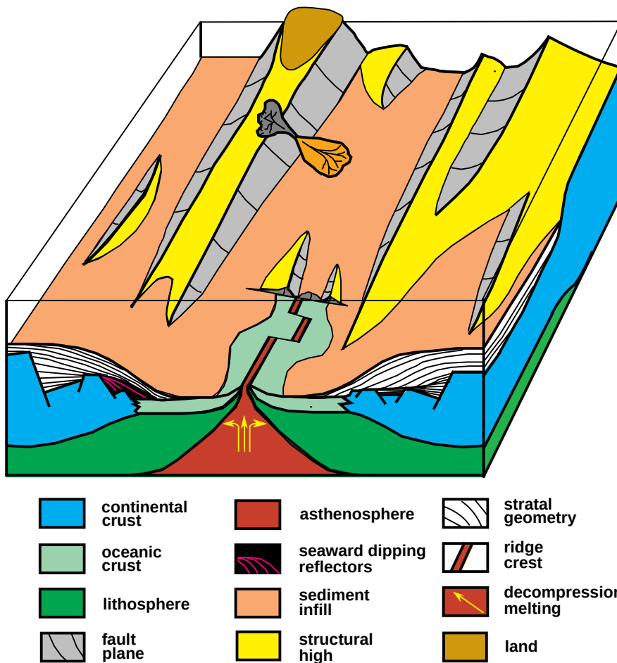
Figure 26. Synthetic view of the processes that rapture continental lithosphere and lead to the formation of rifted margins, associated sedimentary basins, and ultimately to formation of oceanic lithosphere. Drilling at various water depths, at shallow or deep penetration, and with or without a riser is one major component of a full suite of approaches (including 4-D imaging, long-term monitoring, geodetic studies, laboratory experiments, and modeling) that improve our understanding of rifting processes. Figure from Coffin, M. et al., EOS Transactions of the American Geophysical Union, 1998.
